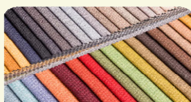
Kubanit
